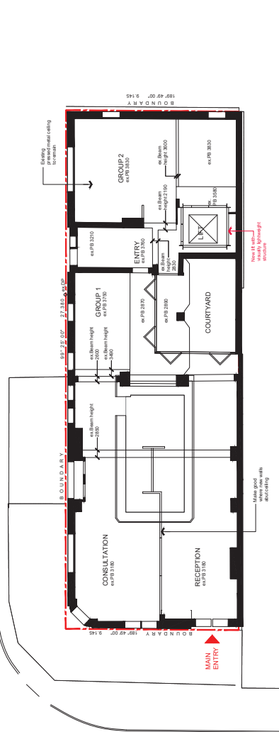
02 REFLECTED CEILING PLAN - GROUND FLOOR Scale 1:100
